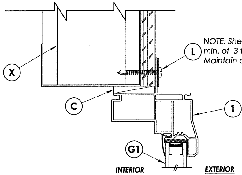
3 3 VERTICAL CROSS SECTION Steel Stud Construction
