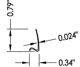
7 GLAZING BEAD
