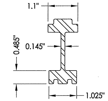
11 MULLION REINFORCEMENT
