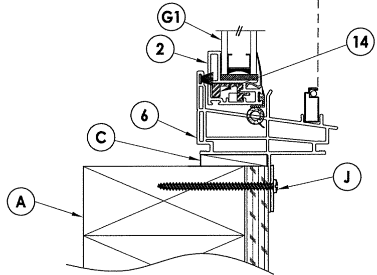
2 3 VERTICAL CROSS SECTION Stud Construction
