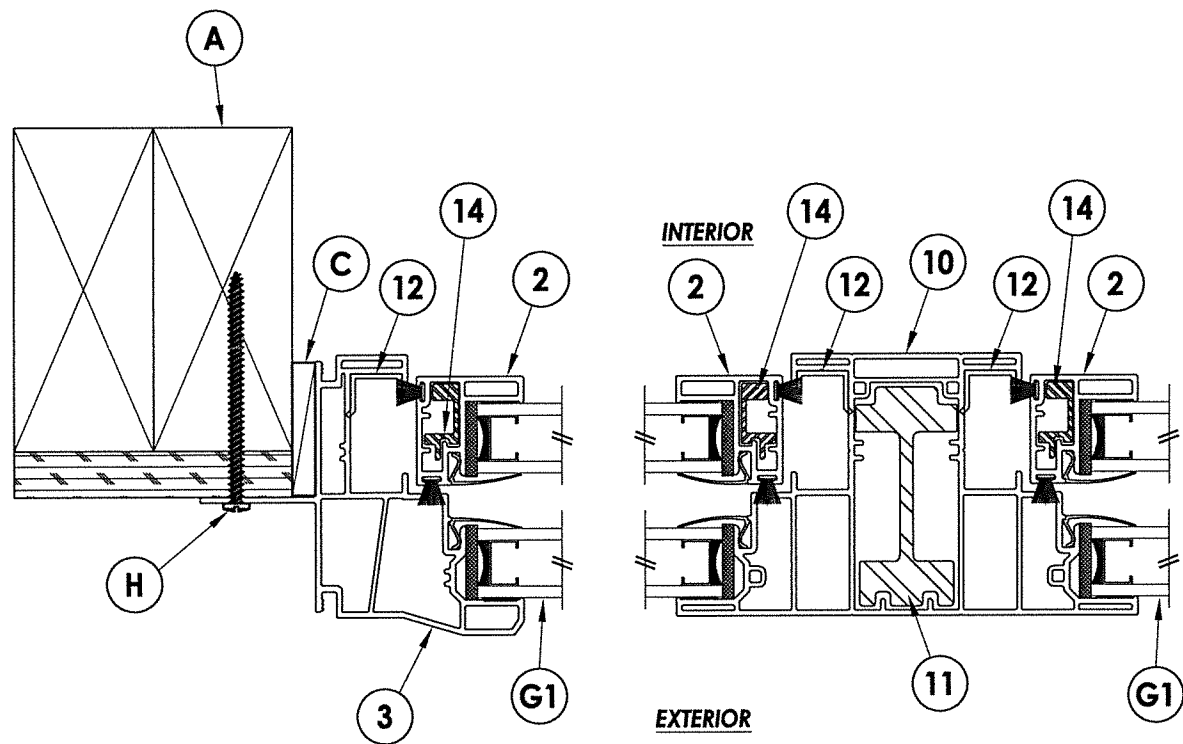
1 3 HORIZONTAL CROSS SECTION Stud Construction
