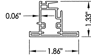
5 MEETING RAIL
