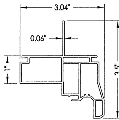
1 FRAME HEAD
