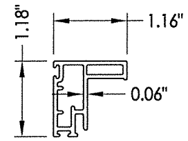
2 SASH STILE/RAIL
